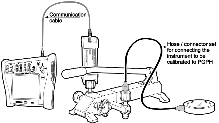
Connections when calibrating a transmitter using an external pressure module.
