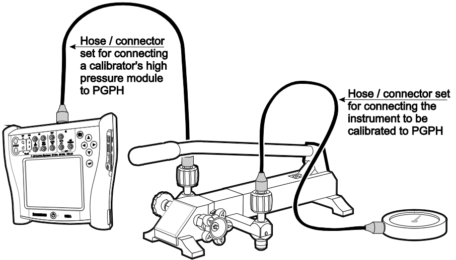
Connections when calibrating a transmitter using an internal pressure module.
